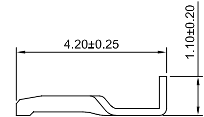
SEC:C-C
