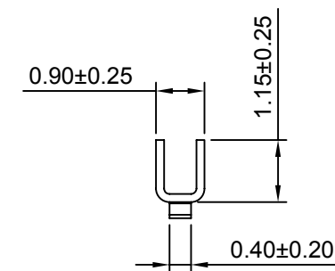
SEC:C-C
